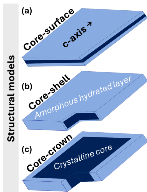
Fig. 3. A diagram illustrating the typical platelet-like structure of CDHA (a) core-surface model; (b) core-shell model; (c) core-crown model. Adapted from [15,42].
