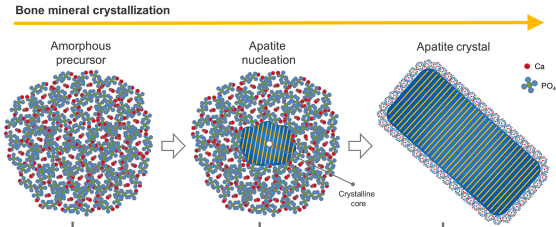
Fig. 16. Schematic of bone mineral crystallization and detection of the conversion of amorphous calcium phosphate (ACP) into apatite. The conversion of ACP into apatite may involve different stages, in which atoms in the center of amorphous particles rearrange into a crystalline core where apatite is nucleated. As the mineral crystallizes, atoms from the ACP component are progressively incorporated into the crystal lattice, leading to the growth of the apatite domain and reduction of the amorphous shell. Taken from [42].
