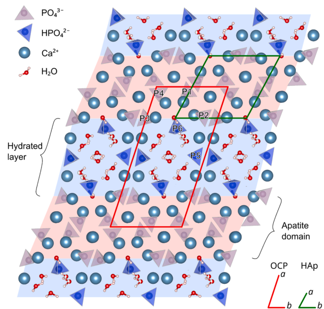
Fig. 2. Crystal structure of triclinic OCP, evidencing the six phosphate groups per unit cell (P1 to P6). The OCP (red) and HA (green) unit cells highlight the structural relationship between the two phases. Adapted from [404]. The lattice parameter “a” in HA (0.954 nm) is 1.6% shorter than the corresponding “b” parameter in OCP (0.97 nm). The “c” parameter of HA (~0.69 nm) corresponds approximately to the thickness of the apatite-like layers in OCP, rather than to the full OCP unit cell parameter. The OCP c-axis (not shown) is associated with the stacking direction of the layered structure and is inclined with respect to the plane of the figure due to the triclinic symmetry.
